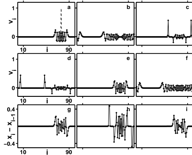
Figure 1. Dispersion vs. solitary waves in a 100 particle chain described by eqs (1) and (2). Axes have been labelled for each row in the leftmost panel with i being the position index of the particle in the chain, v_i its velocity and x_i its displacement from its equilibrium position. In figure 1a and 1b, the initial perturbation (shown in dashed lines) disperses in a harmonic chain, i.e. with \beta = 0 in eq. (2); the perturbation splits up into pairs of compression and dilation waves as shown in the displacement plot in figure 1g corresponding to figure 1a. If \alpha = 0 in eq. (2), we get solitary wave pulses which are shown in figures 1c and 1d, again in pairs of compression and dilation pulses as can be seen from the displacement plot of figure 1h corresponding to figure 1c; note how the primary pulses are well-separated from the subsequent rattling at the site of initial perturbation, from which can be seen emerging secondary solitary wave pulses. If both \alpha, \beta \neq 0 in eq. (2) (see figures 1e and 1f), we have dispersion as the final result albeit controlled by the relative strengths of \alpha and \beta . The displacement plot corresponding to figure 1e is shown in figure 1i.
