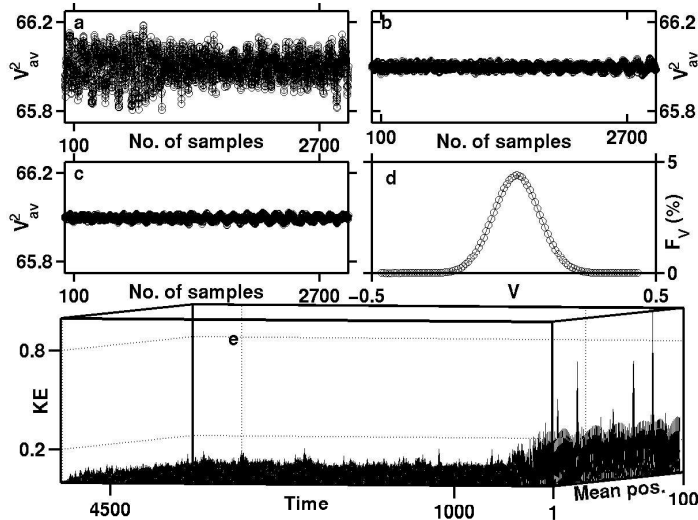
Figure 3. Nature of asymptotic state. The first three panels (figures 3a–3c) show the spatial average of the square of the velocity of the particles, averaged over three different time periods, T = 400 , T = 2000 and T = 3000 , respectively. 3000 samples each are shown, which have been taken from consecutive starting points, after 75,000 time-steps of integration; y -axis has been scaled by 10^4 . Note that, although the fluctuations in the average are quietened down with increasing T , no further smoothing is possible with larger T 's. Figure 3d shows that the velocity distribution over the chain is Gaussian in this state. Figure 3e shows a plot of the kinetic energy of each particle against time, from t = 0 to t = 5000 ; note that the system reaches quasi-equilibrium very fast.
