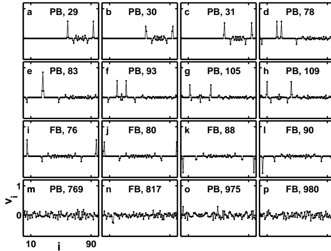
Figure 2. Collisions of solitary waves between themselves as also with walls. Axes have been labelled in panel m , and remains the same for all others; i is an index to the position of the particle in the 100 particle chain, and v_i its velocity. PB/FB indicates periodic/fixed boundary conditions, and the numbers next to them give the time after initial perturbation. figures 2a–2c show the ‘breathing’ feature of the discrete chain as the solitary wave steps over the adjacent particles in its motion along the chain. The two primary pulses from the site of initial perturbation, in a chain with periodic boundaries, ‘pass through’ each other in figures 2d–2f leaving behind some energy at the site of the collision (figure 2f) in the form of prolonged rattling from which will emerge, subsequently, secondary solitary wave pairs, similar to the ones from the site of initial perturbation seen in earlier panels. The primary solitary waves meet up with the secondary ones from the site of initial perturbation and pass through each other in figures 2g and 2h. In figures 2i–2l, we show the collision of primary solitary waves from the site of initial perturbation, in a chain with fixed boundaries, with the walls at either ends, and their reflection with hardly any loss of energy. The panels in figures 2m–2p show the qualitatively similar, noisy, state of the chain, in both periodic and fixed boundary cases, in the asymptotic state after numerous collisions.
