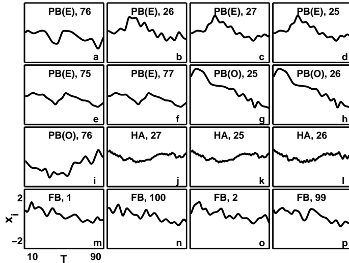
Figure 4. The figure shows correlations induced by boundary conditions. PB and FB refer to periodic and fixed boundary conditions, respectively. E and O further distinguish between chain with even number of particles ( = 100 ) and odd number ( = 101 ) of particles, respectively. HA refers to chain with only harmonic potential, even number of particles ( = 100 ) and periodic boundary conditions. The particle numbers are indicated next to these labels. Oscillations of selected particles over a time period of T = 100 arbitrary units, in the steady state are shown. Axes in all panels are as in figure 2.m; x_i is the displacement of the i th particle from equilibrium position. figures 2.a and figure 2.b show the two particles at the equatorial points diagonally across (see eq. (3)), which both have their own unique dynamics. Particles on either side of these equatorial particles are (separately) synchronized as shown in figures 2.c–f. In the case of odd number of particles in a chain with periodic boundaries, only N_{eq} has its unique dynamics, while its diagonally opposite particle at the equator is now paired off with another in synchronized dynamics (figures 2.g–h); rhythms of N_{eq} are shown in figure 2.i. The next three panels (figures 2.j–l) show that a similar situation to that with quartic potentials is obtained in a harmonic chain with periodic boundaries; synchronized rhythms of particles sitting across one of the equatorial particles are shown in figures 2.j and k and the unique rhythm of the corresponding equatorial particle is shown in figure 2.l. In the case of the chain with fixed boundaries, one does not see such synchronizations, as shown with the particles next to the walls and adjacent to those (figures 2.m–p) in a 100 particle chain.
